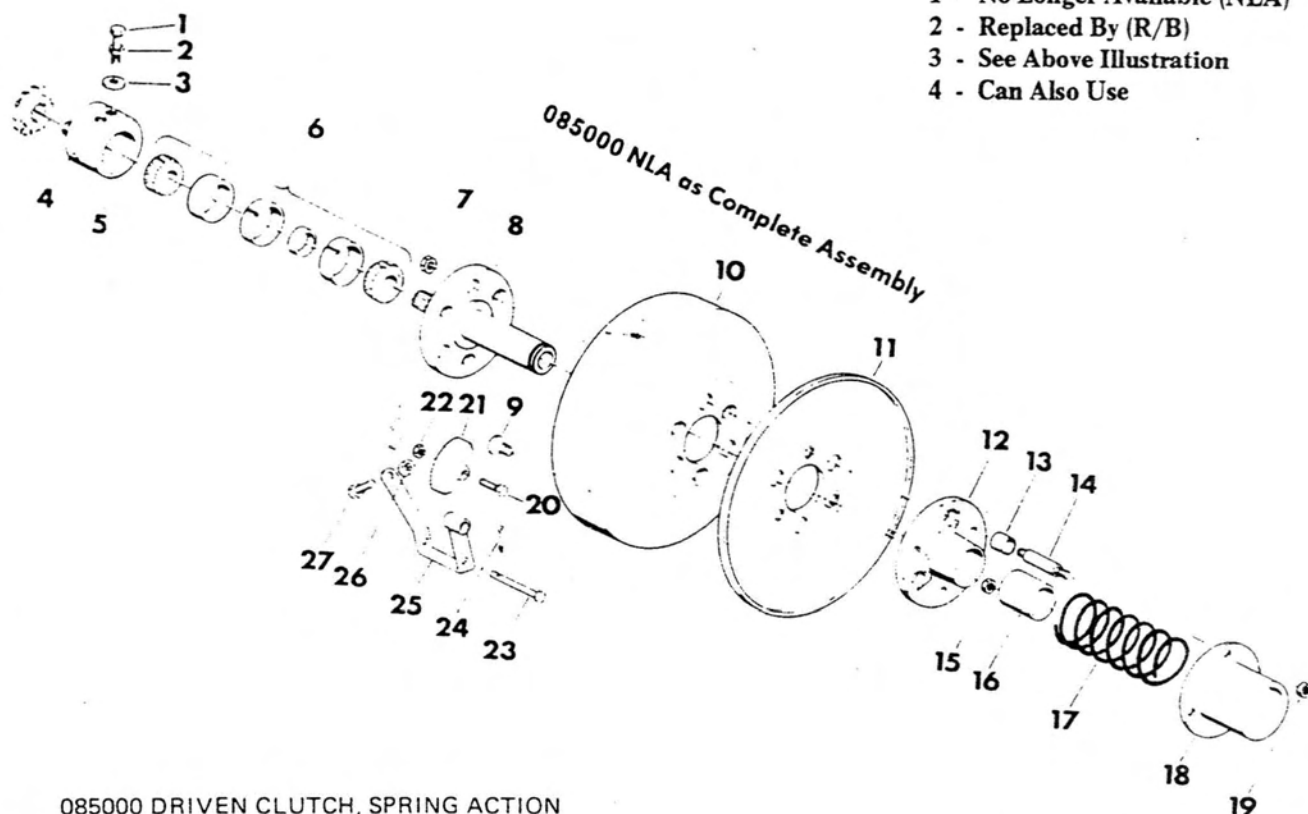
085000 DRIVEN CLUTCH, SPRING ACTION
