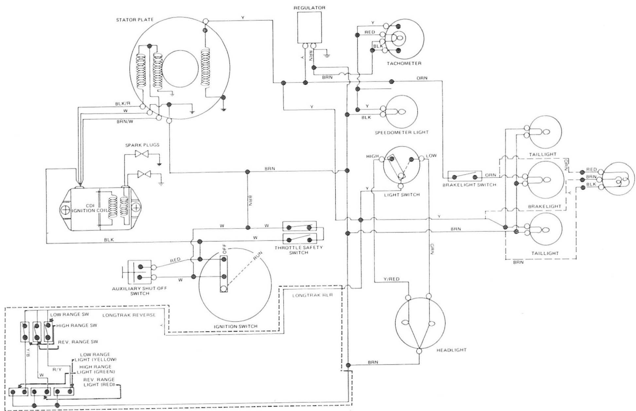
1988 SCHEMATIC DIAGRAM
