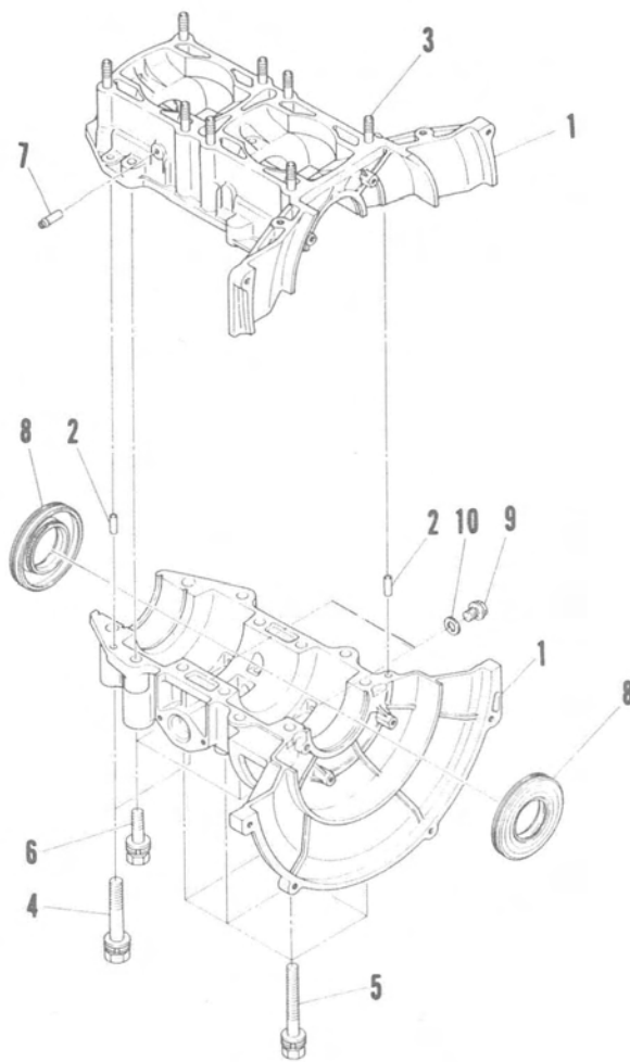
Crankcase
