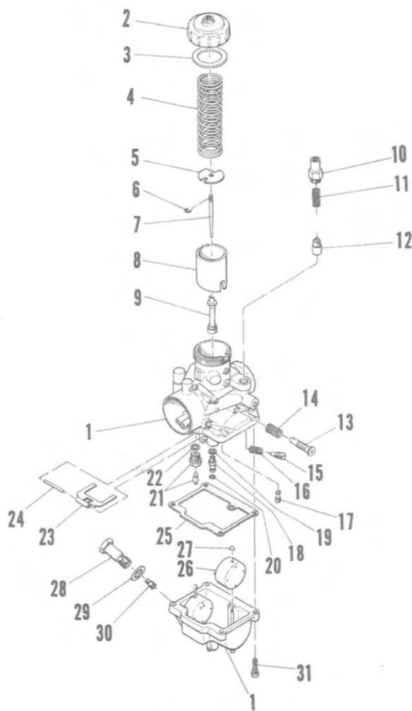
Carburetor
