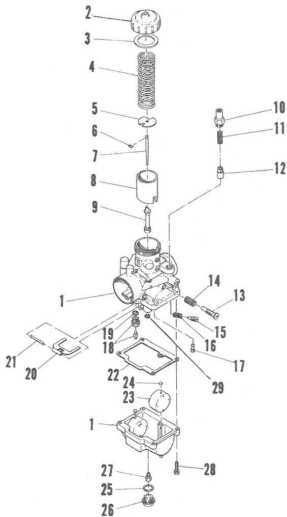
Carburetor (Trail and 400)
