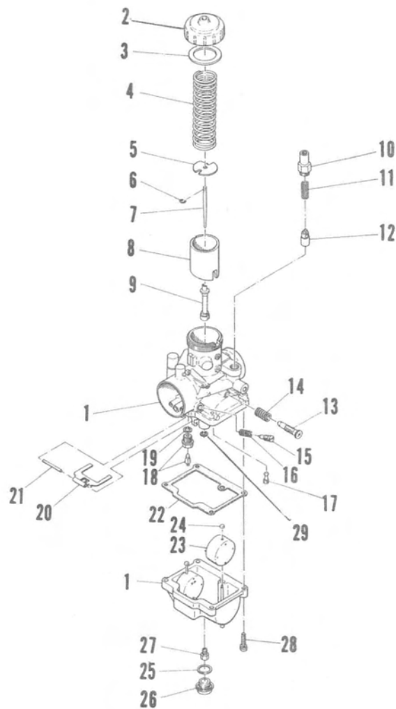
Carburetor (400)
