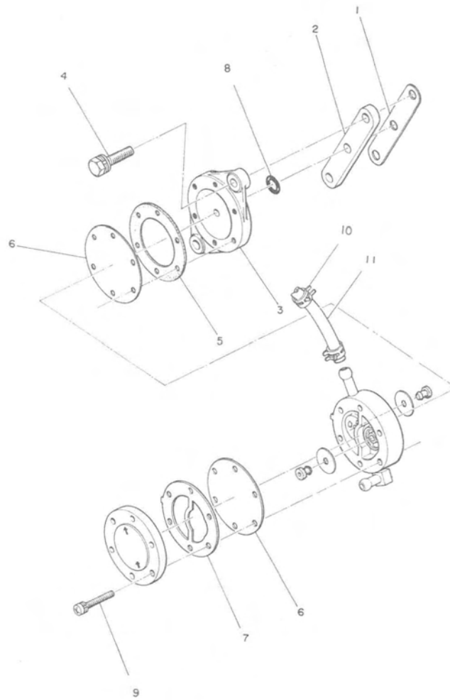
Fuel Pump (Star LT)
