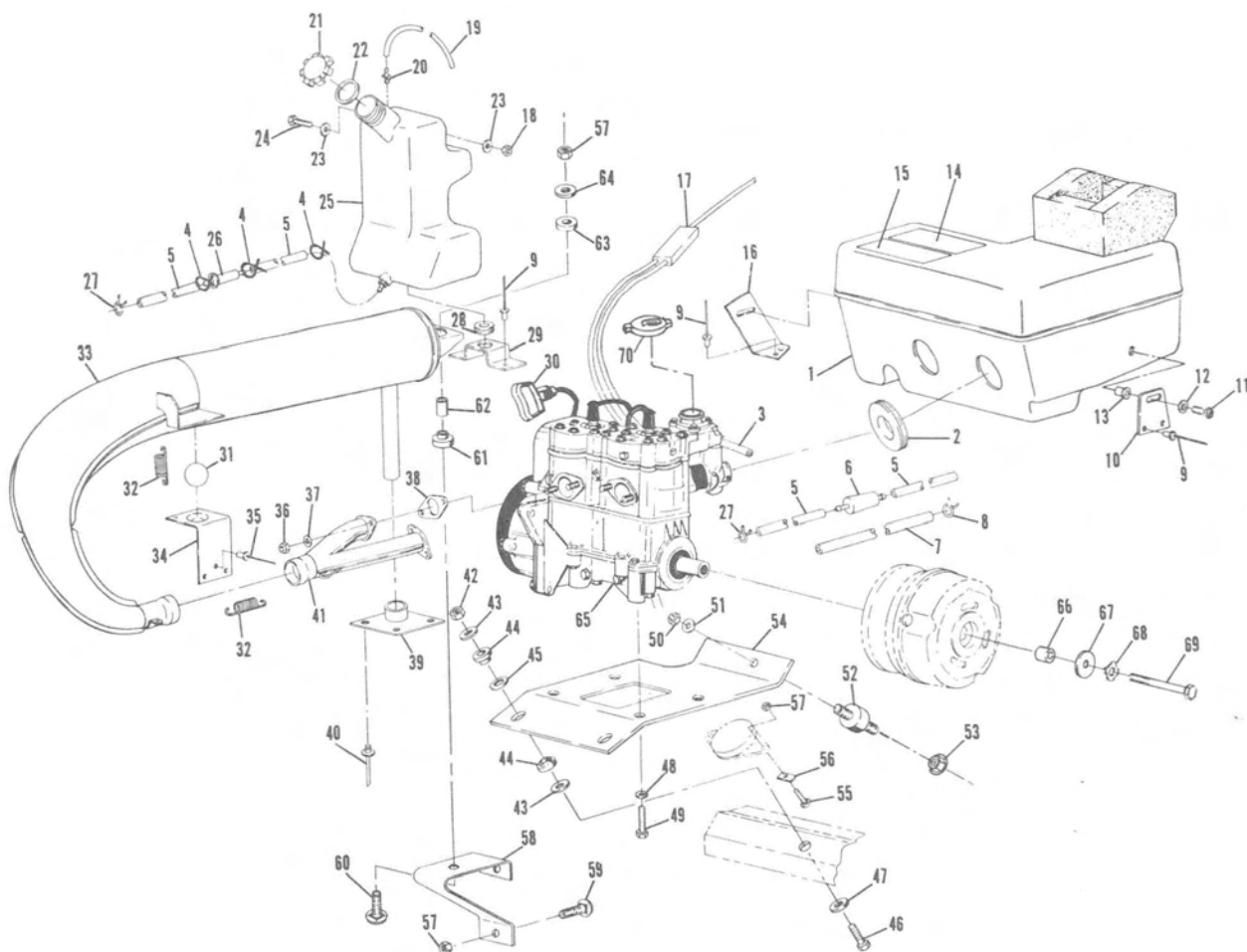
Engine Mounting (400)
