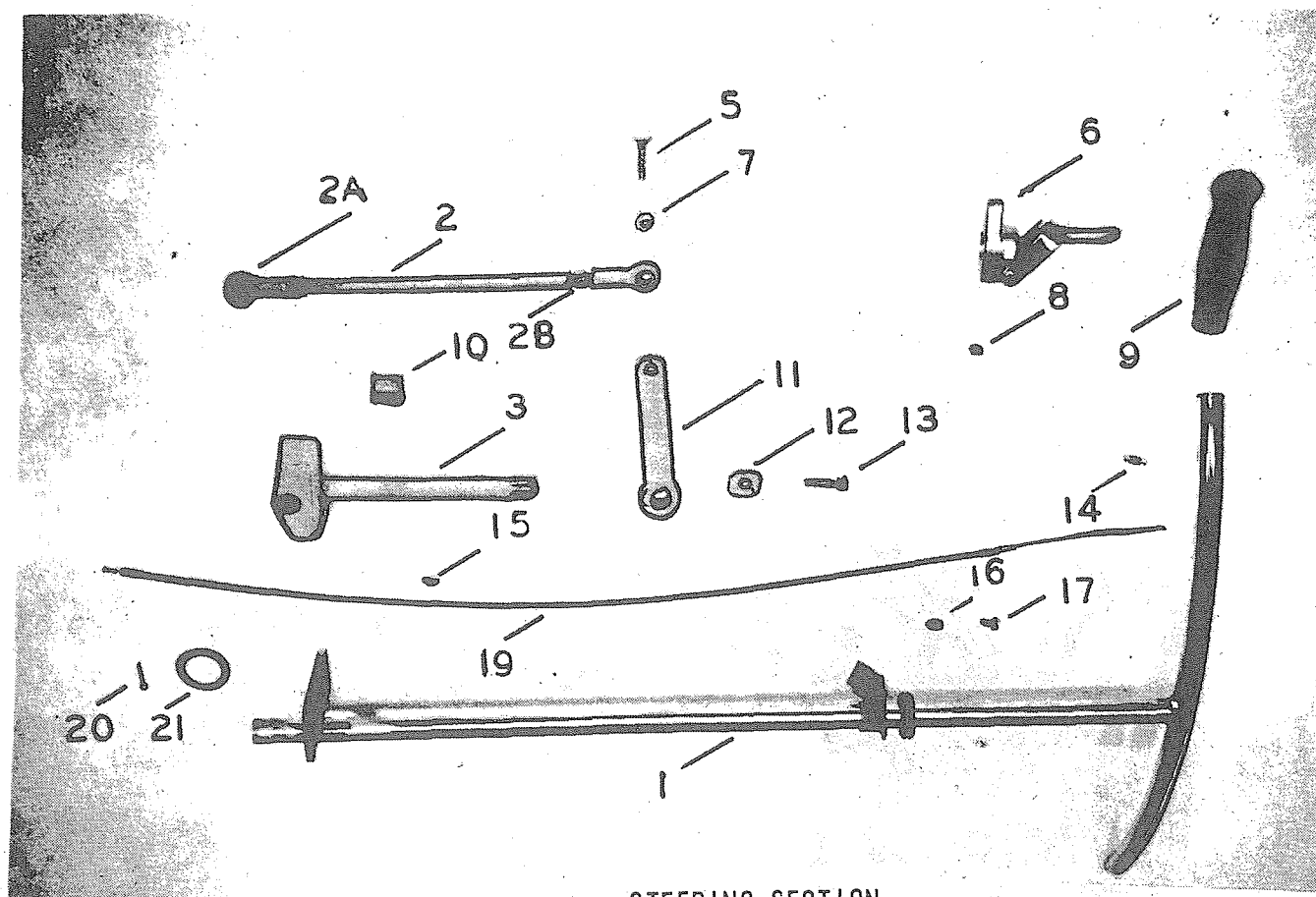
STEERING SECTION
