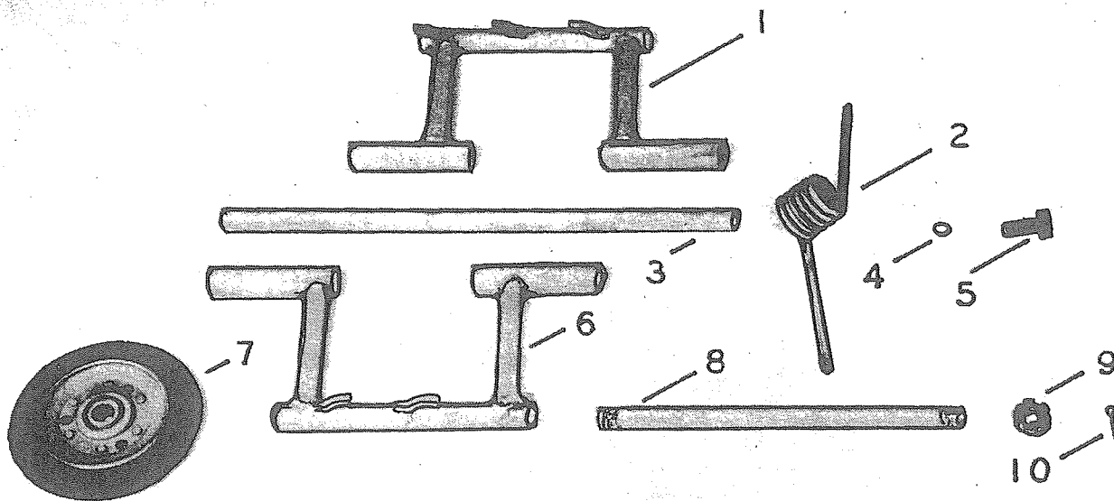
BOGIE ASSEMBLY
