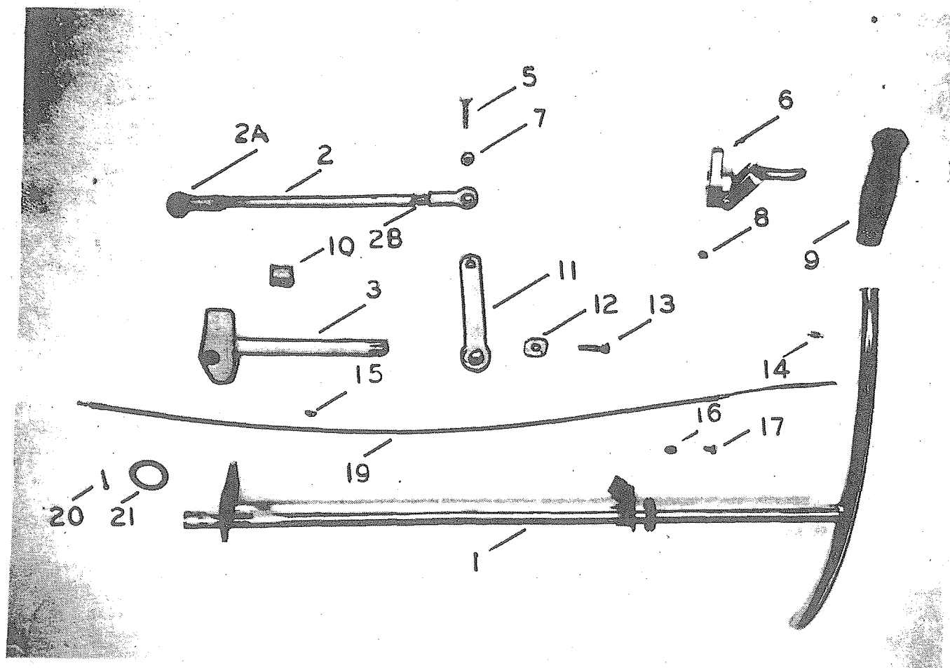
STEERING SECTION
