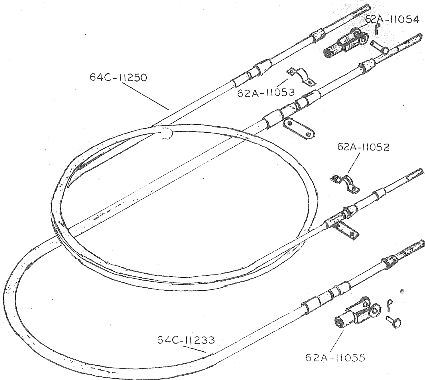
Throttle & Brake Cable
