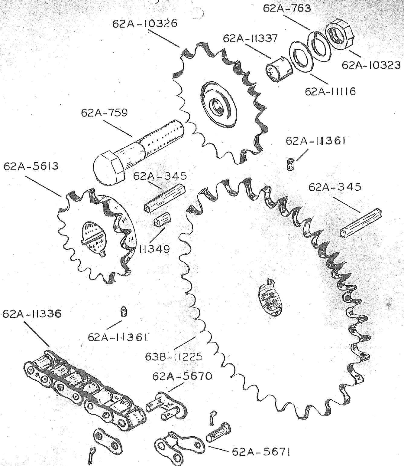
Rear Drive Sprockets & Idler Sprocket
