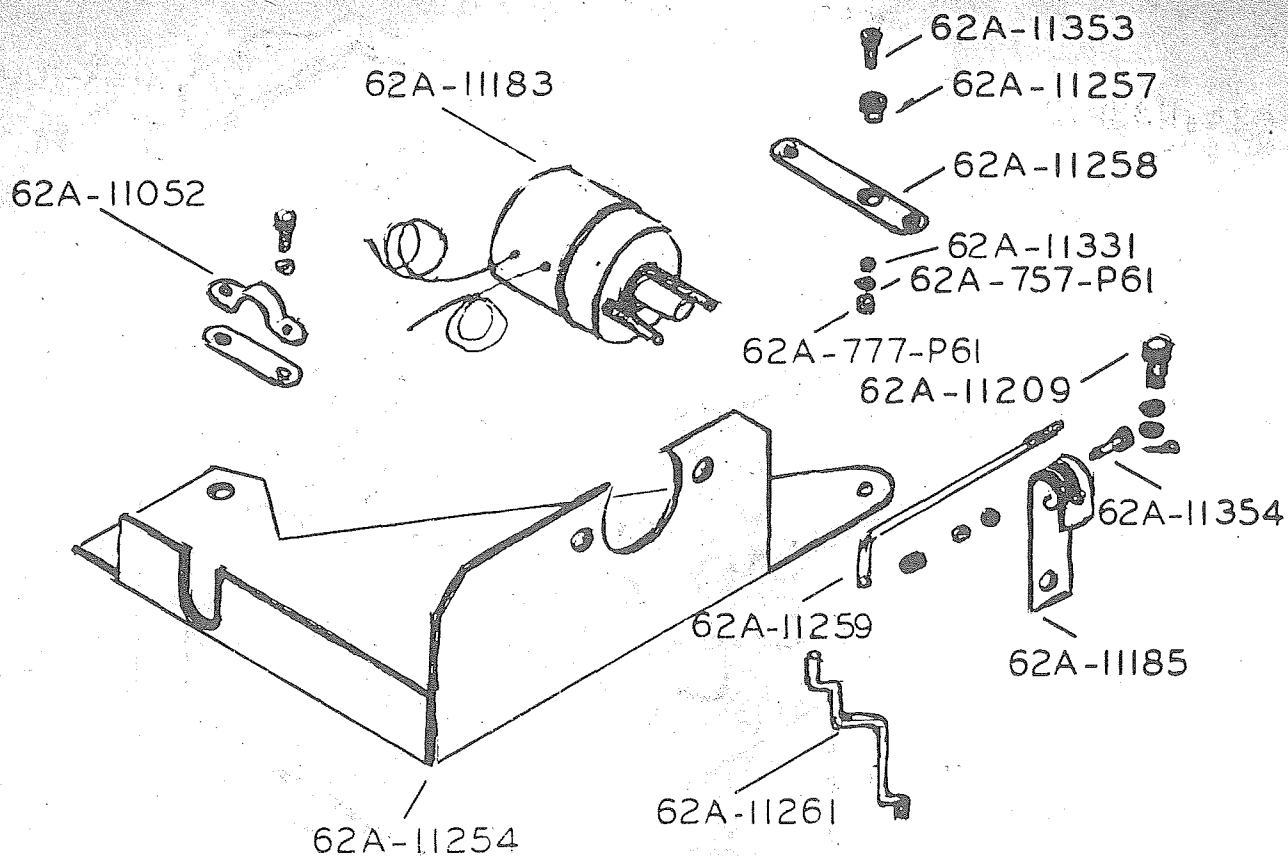
Solenoid & Bracket
