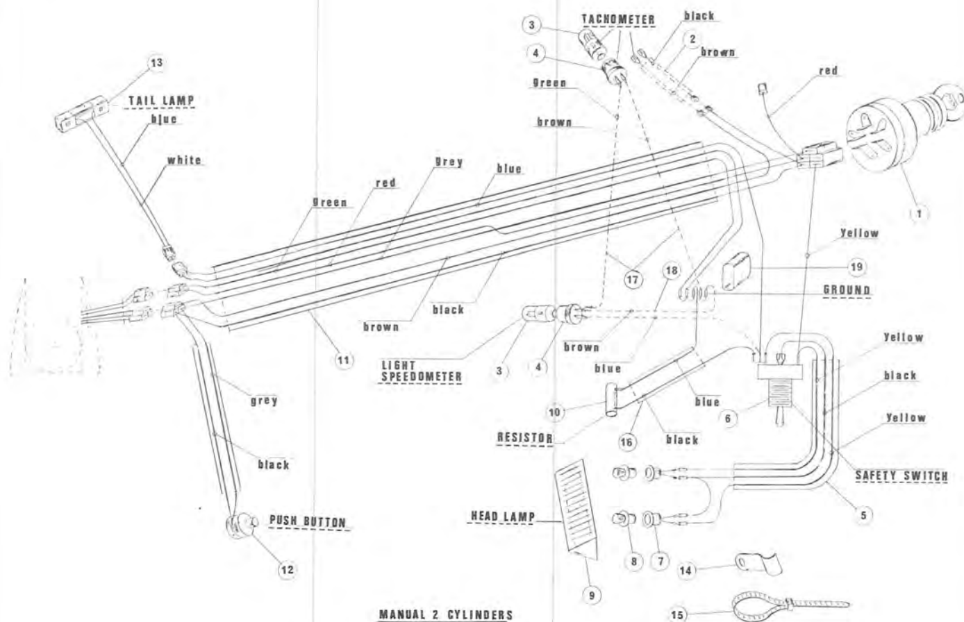
MANUAL 2 CYLINDERS
