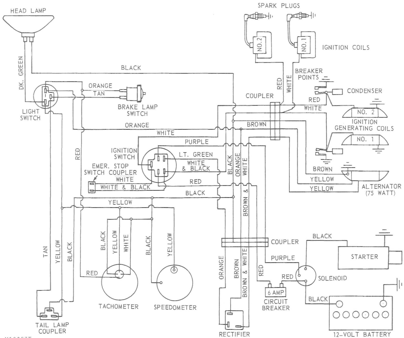
Fig. 2-Wiring Diagram with Electric Start 400 and 500 Snowmobiles (Serial No. 2551-11,000)
