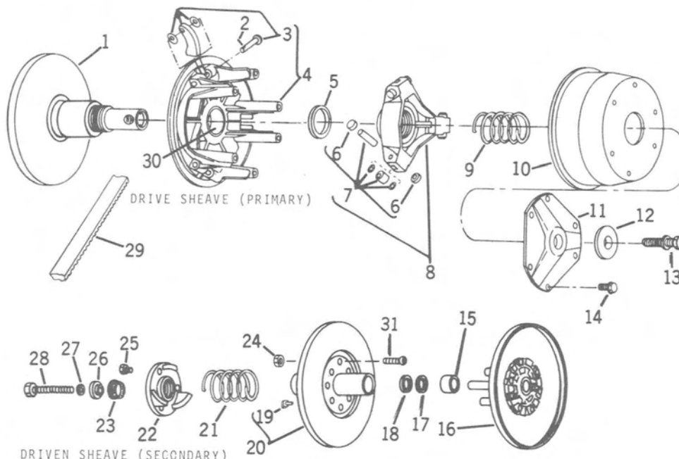
M20639F DRIVEN SHEAVE (SECONDARY)
