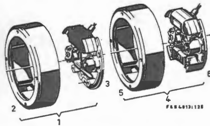
Magneto-generator
