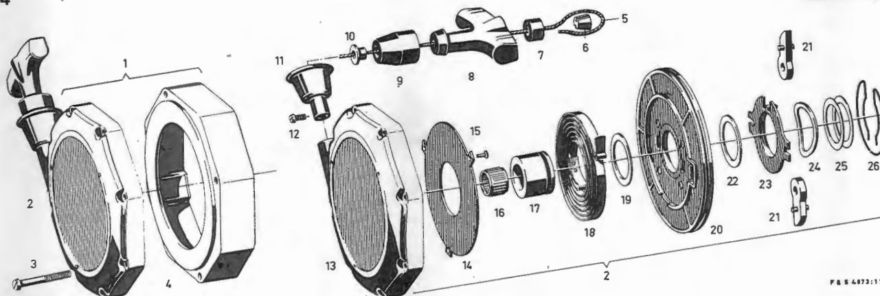
Recoil starter
