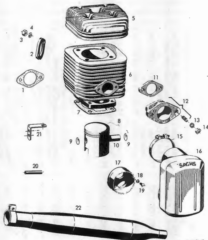
Plate 13 Conversion kit for competition engine SA 320, designed on the basis of the SA 290
