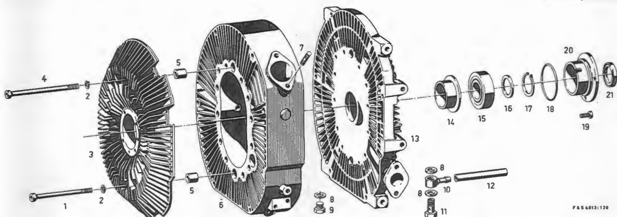
Short exchange engine
