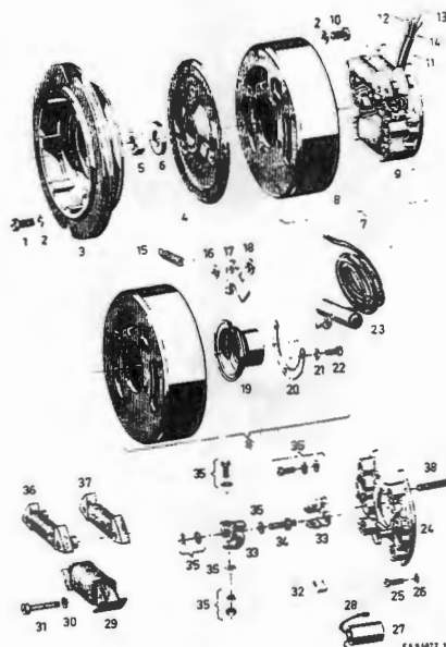
Magneto-generator 12 V - 40 W
