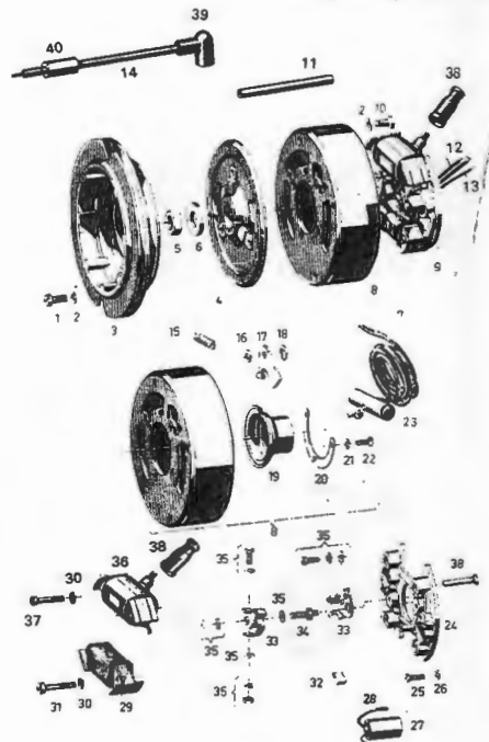
Magneto-generator 12V - 40W
