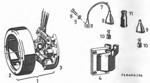
Magneto-generator with ignition coil fitted outside of the engine
