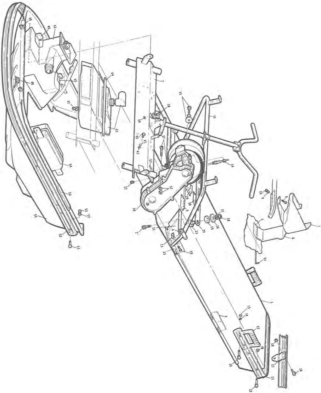
Figure 2. Chassis and Pan Assembly
