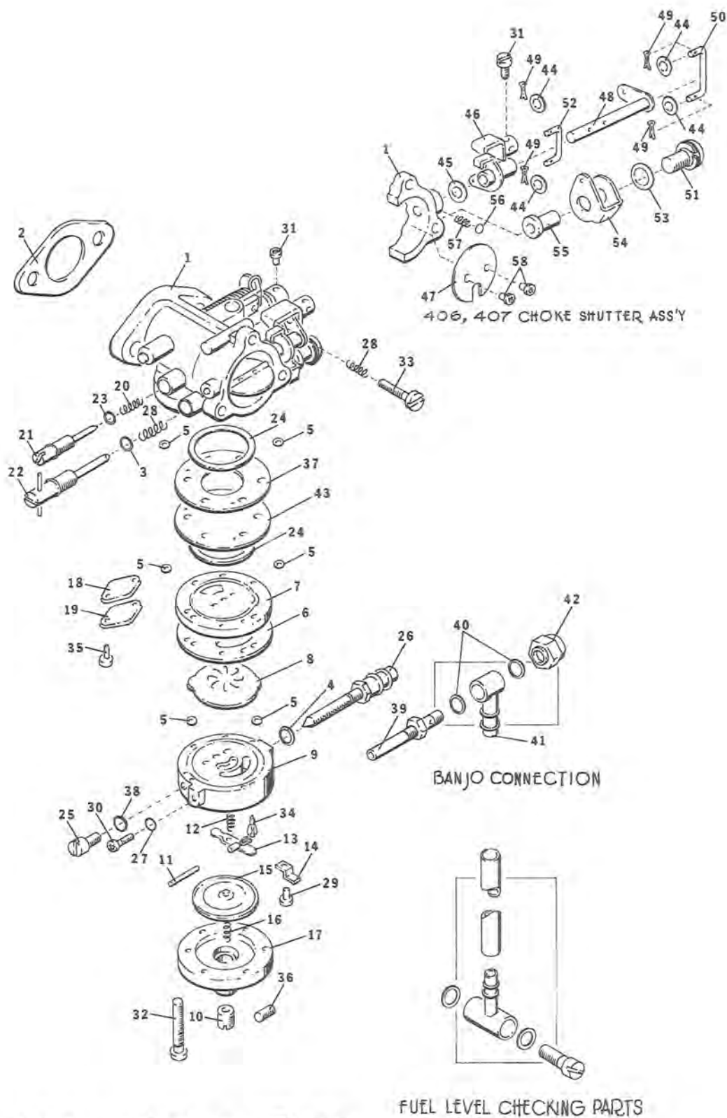
Figure 5-5 Carburetor Assembly
