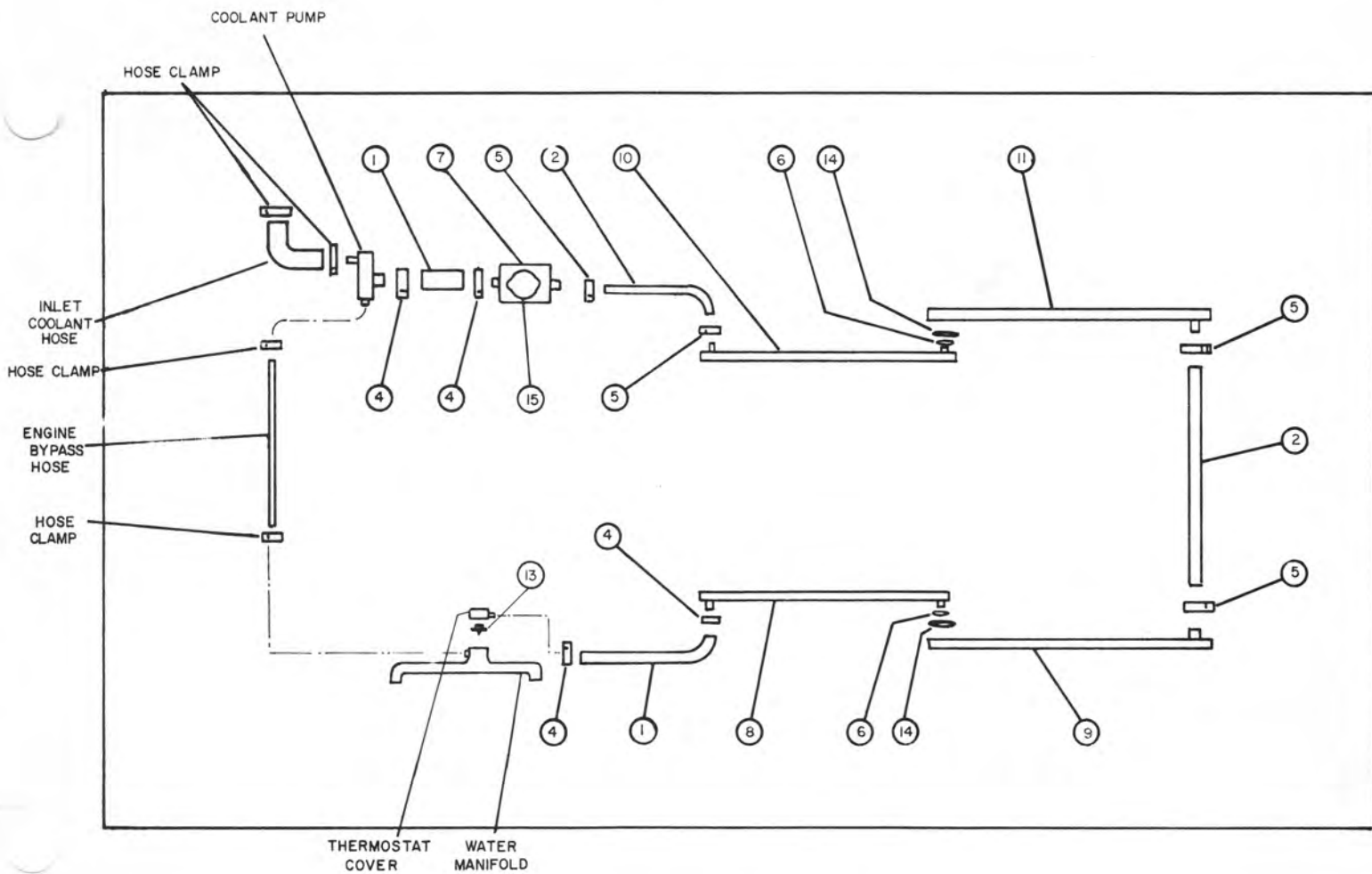
1973 COOLING SCHEMATIC
