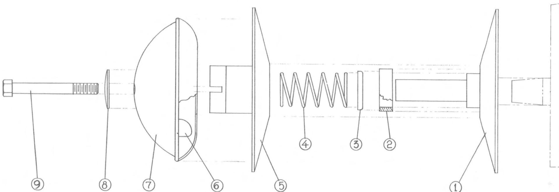
10) COMPLETE DRIVE CLUTCH
